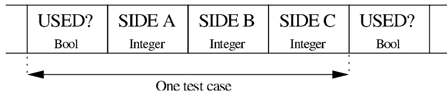
Figure 24: A single test case for the triangle problem [SF96]
