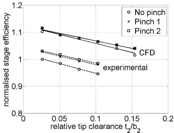
Fig. 5. Measured and modelled stage efficiency.
