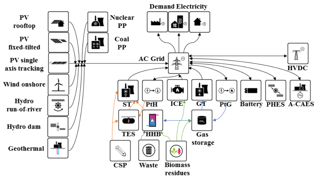
Figure 4. Block diagram of the LUT Energy System Transition model used for South Africa (Breyer et al., 2018). Abbreviations not introduced elsewhere include PP- power plant, ST- steam turbines, PtH – power-to-heat, ICE – internal combustion engine, GT gas turbines, A-CAES – adiabatic compressed air storage,
