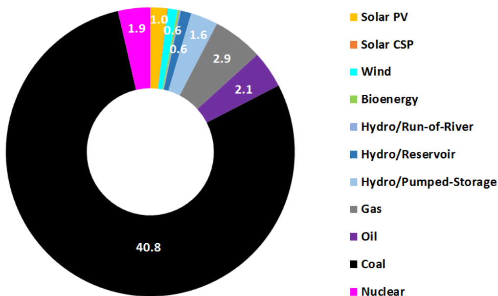
Figure 1. Total installed active power capacities (in GW) by the end of 2014 in South Africa (Farfan and Breyer, 2017).
