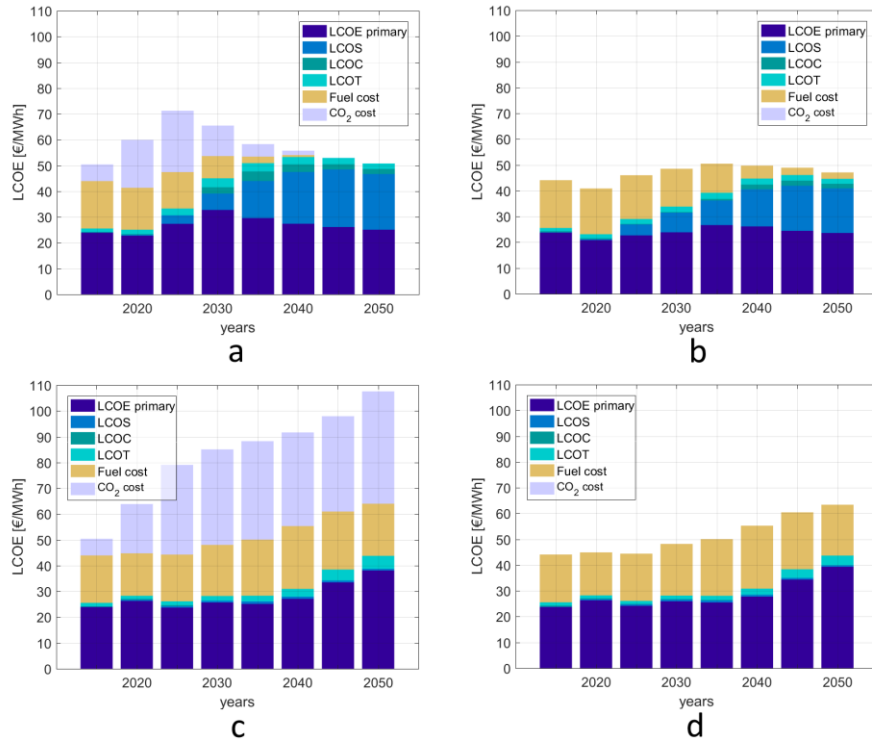
Figure 7. Levelised cost of electricity for BPS (a), BPSnoCC (b), CPS (c), and CPSnoCC (d).
