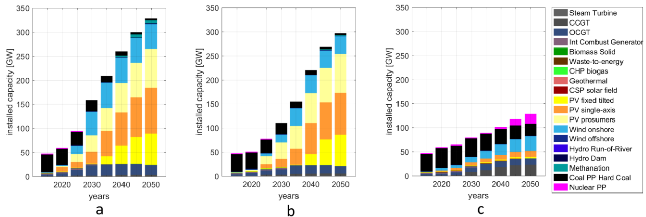
Figure 8. Installed generation capacities for BPS (a), BPSnoCC (b) and CPS (c) from 2015 to 2050.
