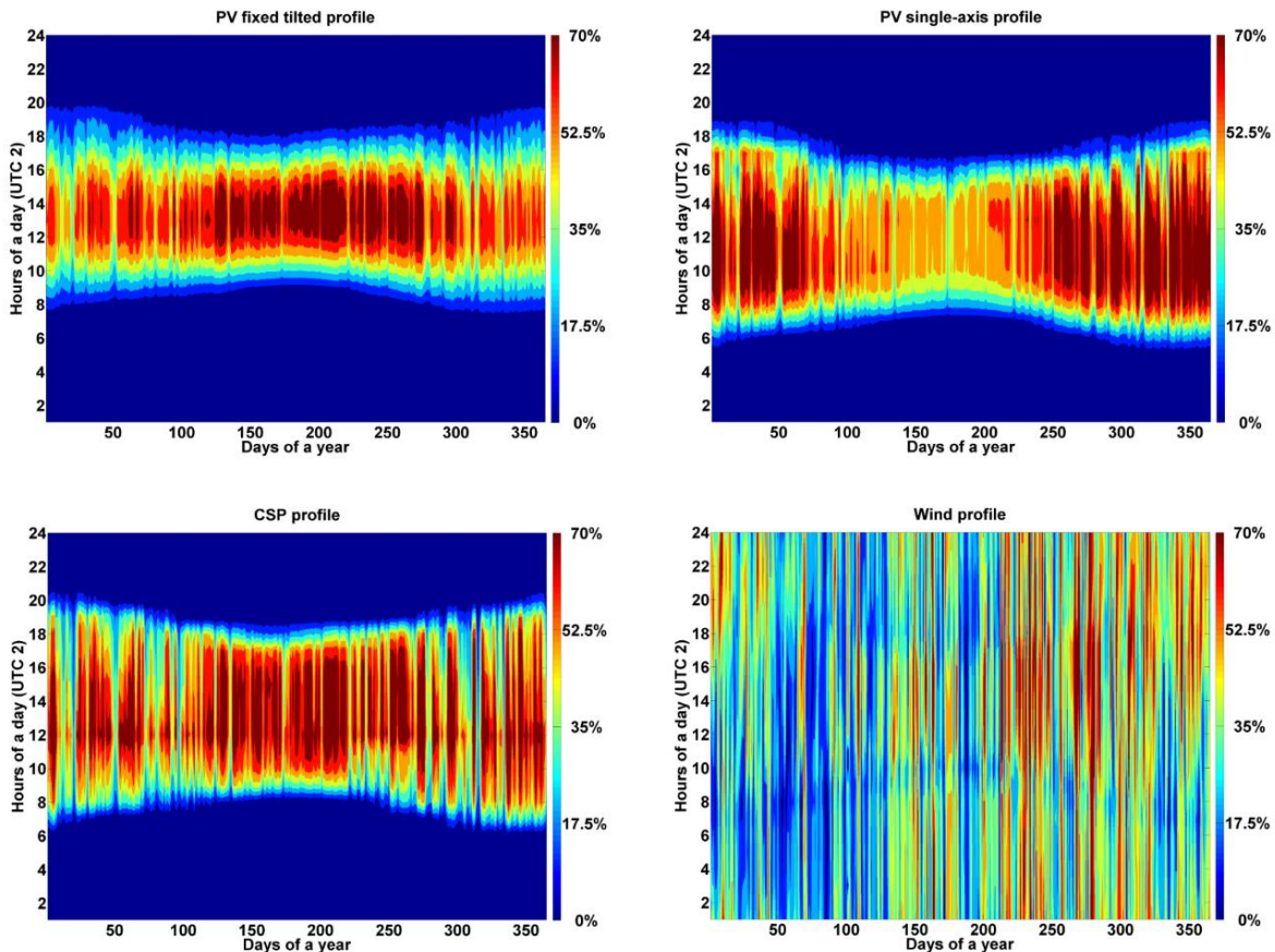
Figure 5. Aggregated feed-in profiles for optimally tilted (top left) and single-axis tracking PV (top right), CSP solar field (bottom left), and wind power plants (bottom right) in South Africa.
