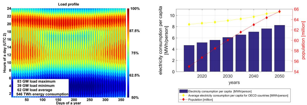
Figure 6. Aggregated load curve for South Africa for 2050 (left) and long-term demand from 2015 to 2050 (right).
