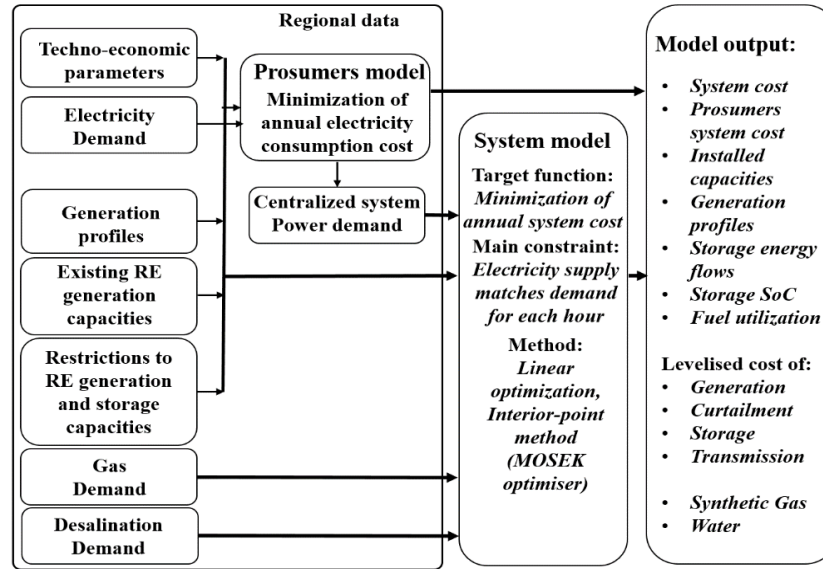
Figure 2. Main inputs and outputs of the LUT Energy System Model (Bogdanov and Breyer, 2016).
