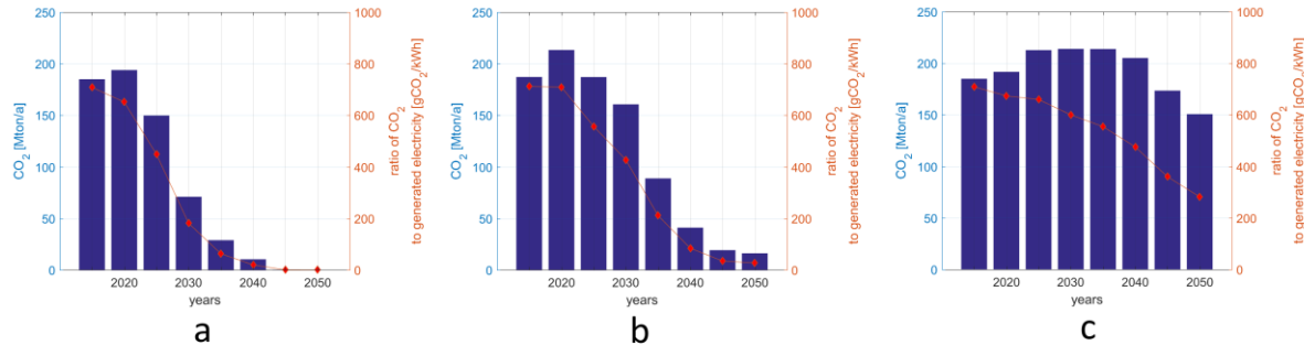
Figure 15. The total annual GHG emissions and ratio of GHG emissions to electricity generation during the transition for BPS (a), BPSnoCC (b) and CPS (c).
