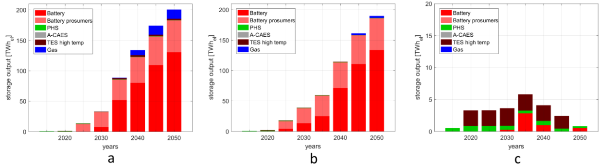
Figure 11. Cumulative storage output for BPS (a), BPSnoCC (b) and CPS (c) from 2015 to 2050.
