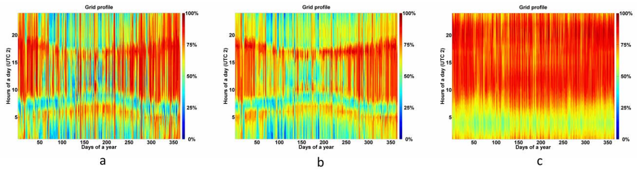
Figure 12. Grid profile for BPS (a), BPSnoCC (b) and CPS (c) for 2050. (Grid profile is the hourly distribution of electricity demand over the entire year)
