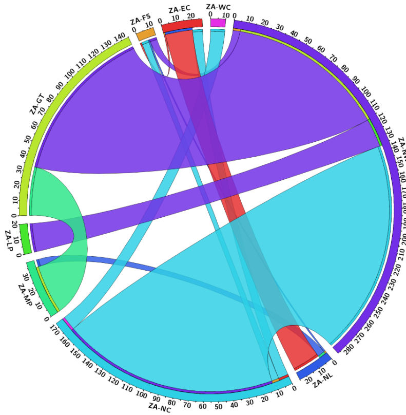
Figure 13. Electricity transmission between the sub-regions for 2050 in the BPS
