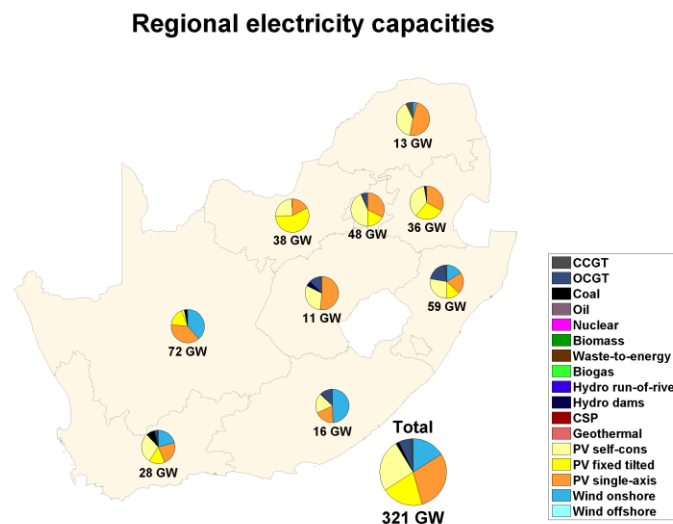
Figure 14. Installed generation capacities for BPS across the nine sub-regions of South Africa for 2050.
