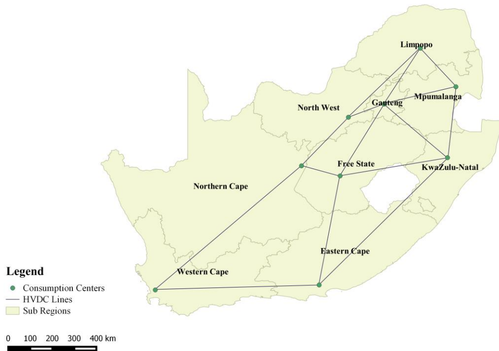
Figure 3. South African sub-regions and transmission lines configuration.
