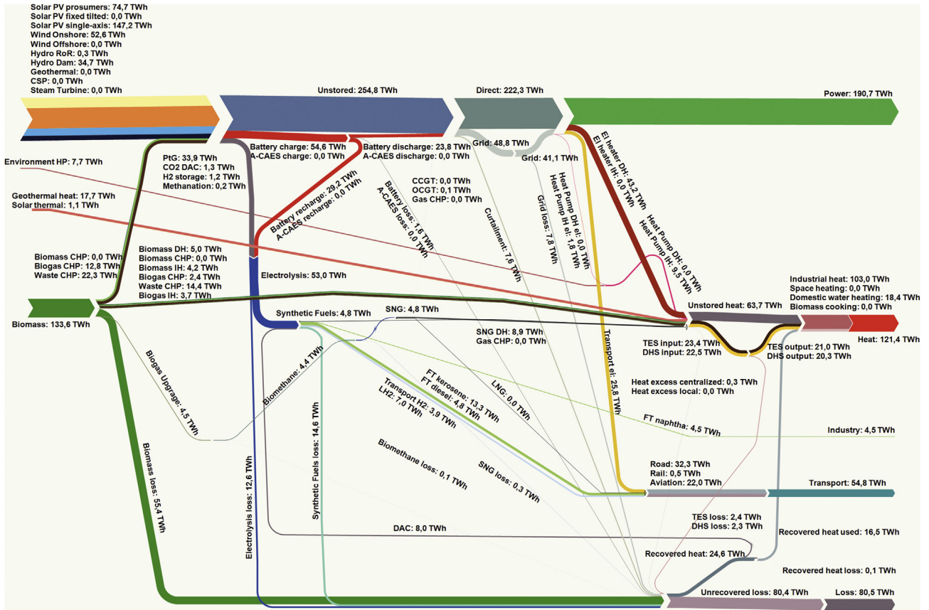
Fig. 21. Energy flow of the system in 2050 for BPS-1. All numbers displayed are in TWh.
