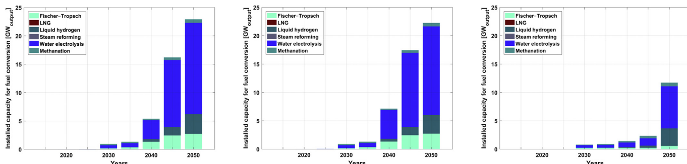
Fig. 17. Total installed capacity for fuel conversion for BPS-1 (left), BPS-2 (centre) and CPS (right) during the transition.
