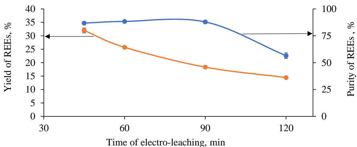
Figure 2. Yield and purity of REEs in cathodic deposit during electro-leaching of spent NdFeB magnet in a mixture of 0.5 M \text{H}_2\text{SO}_4 and 0.05 M \text{H}_2\text{C}_2\text{O}_4 at 50 \text{A/dm}^2 .
