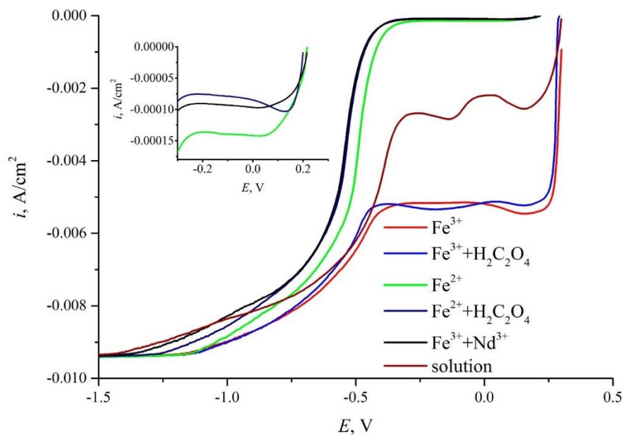
Figure 9. Linear polarization curves of synthetic solutions ( c_{Fe} = 10 g/L and c_{Nd} = 2 g/L) and a leaching solution obtained after 1 h electro-leaching. Insert shows the initial part of Fe^{2+} reduction curves.
