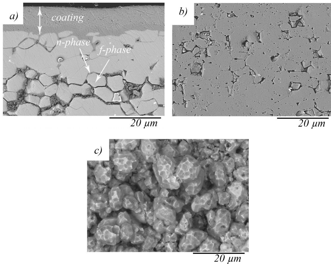
Figure 4. SEM images of the spent NdFeB magnet surface initially (a), after 10 s etching in 1 M HNO 3 (b) and after 1 h electrochemical leaching in a mixture of 0.5 M H 2 SO 4 and 0.05 M H 2 C 2 O 4 at i=50 \text{ A/dm}^2 (c)
