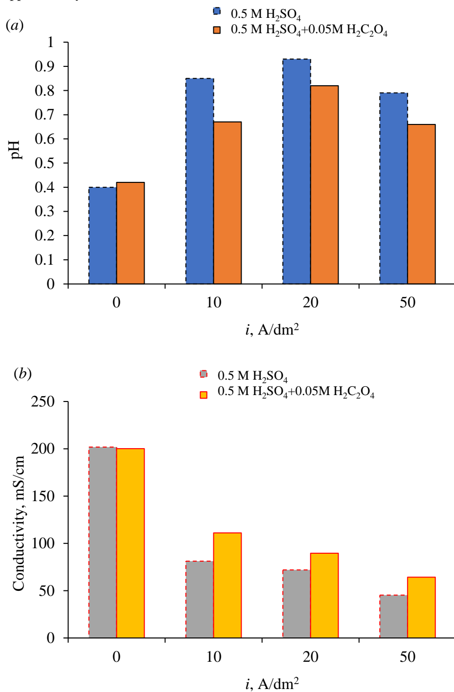
Fig 1S. Effect of current density on pH (a) and conductivity (b) of solution obtained in \text{H}_2\text{SO}_4 and mixture of 0.5 M \text{H}_2\text{SO}_4 and 0.05 M \text{H}_2\text{C}_2\text{O}_4 after 1 hour of electrolysis ( i=0 means initial solution)
