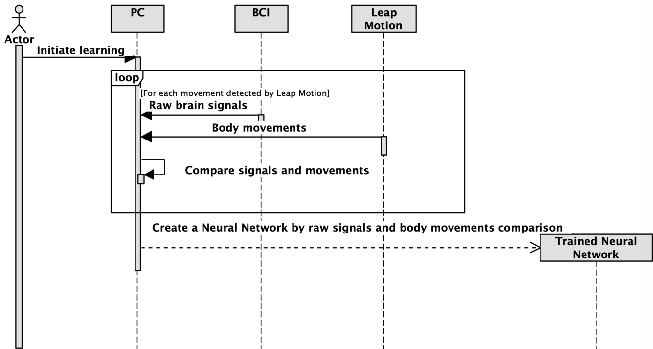
Fig. 4. BCI learning process
