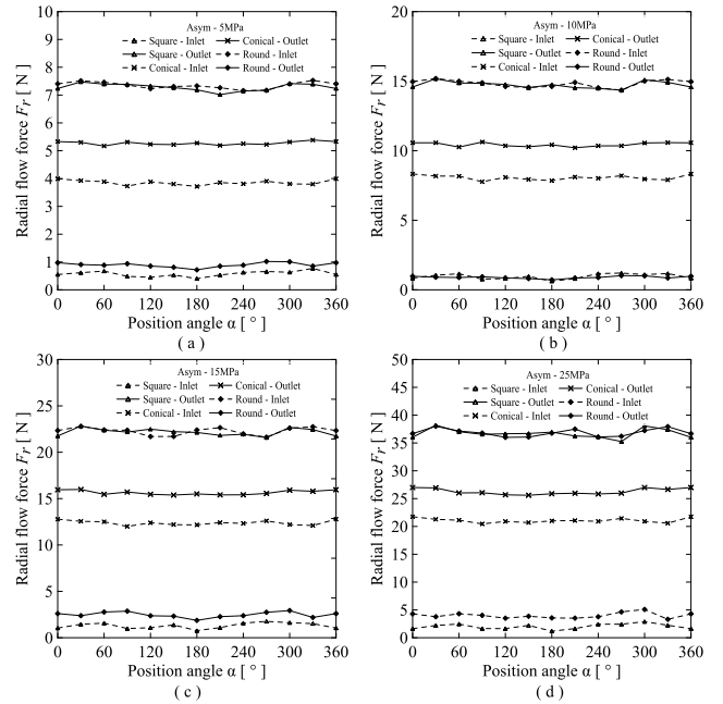
FIGURE 11. Radial flow force variations of three profiles, inlet and outlet control modes, and four pressures when the oil ports are asymmetric. (a) 5 MPa, (b) 10 MPa, (c) 15 MPa, (d) 25 MPa.
