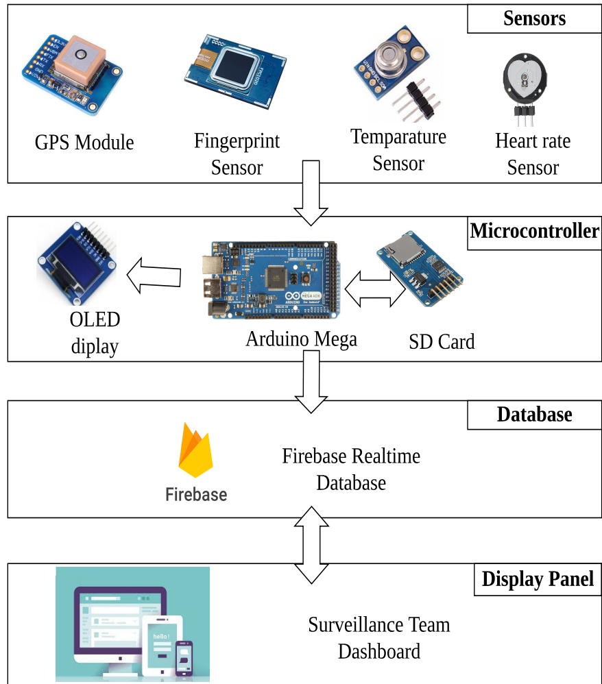
Fig. 3: A layered architectural view of system components
