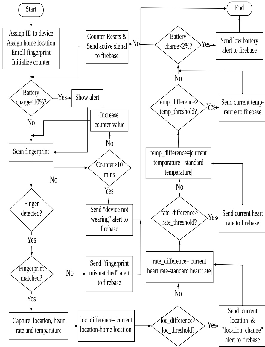
Fig. 4: System workflow diagram
