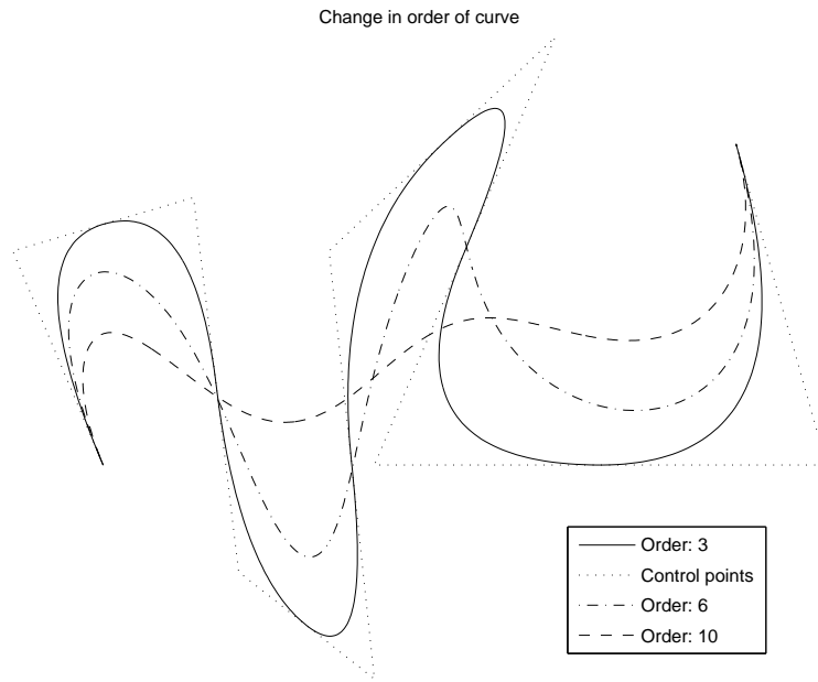
Figure 4. Influence to the shape of curve when changing the order of the curve. For the curve which order is three the knot vector is the same as in Example 1. The knot vector for the curve with order 6: U = \{0, 0, 0, 0, 0, 0, \frac{1}{5}, \frac{2}{5}, \frac{3}{5}, \frac{4}{5}, 1, 1, 1, 1, 1, 1\} . The knot vector for the curve with order 10: U = \{0, 0, 0, 0, 0, 0, 0, 0, 0, 0, 0, 1, 1, 1, 1, 1, 1, 1, 1, 1, 1, 1\} .
