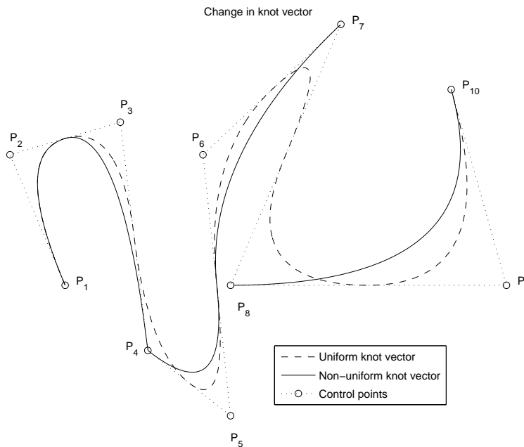
Figure 5. Influence of the change in the knot vector to the shape of curve. In the curve with a uniform knot vector the parameters are same as in Example 1. Only change between the curves is that the second one has a non-uniform knot vector. The non-uniform knot vector of the curve in this figure is: U = \{0, 0, 0, \frac{1}{8}, \frac{2}{8}, \frac{2}{8}, \frac{4}{8}, \frac{6}{8}, \frac{6}{8}, \frac{6}{8}, 1, 1, 1\} .
