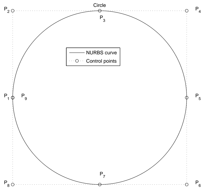
Figure 7. Perfect circle: created using NURBS.
