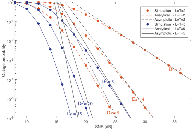
Fig. 3. Exact and asymptotic outage probability curves for massive MIMO-NOMA system operating with the proposed SSAA technique ( N = 4 ).
